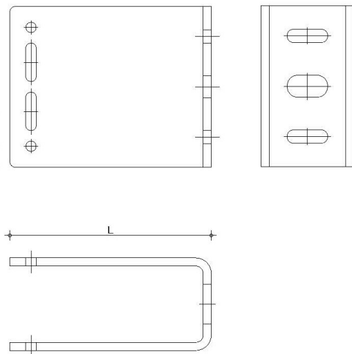
EVT II U Bracket A2 60 x 180mm Stainless Steel
