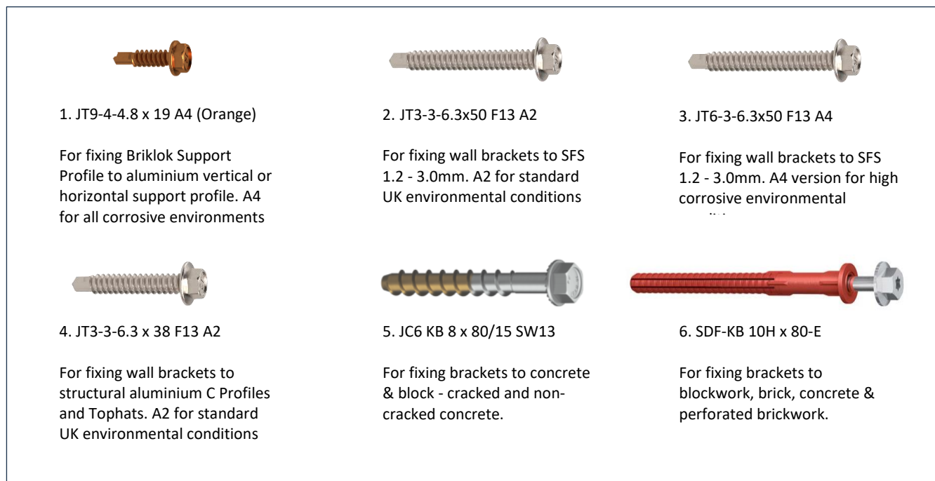
EVT II System ETA fixing examples for steel, concrete & masonry.
