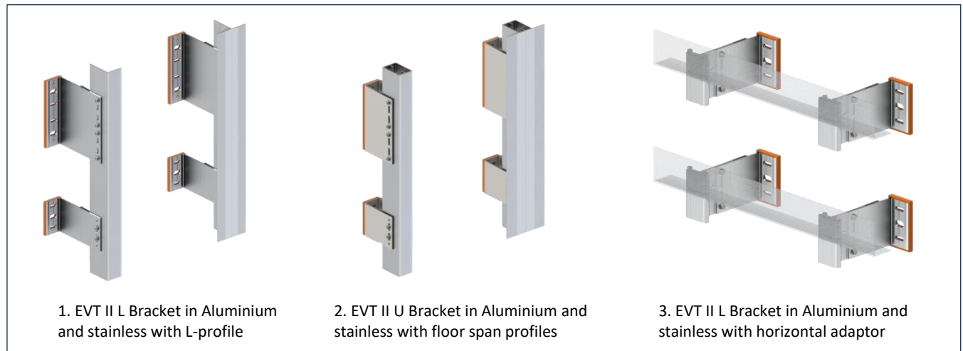
Typical RJ Façade System - EVT II support structure assemblies for supporting Briklok profiles.
